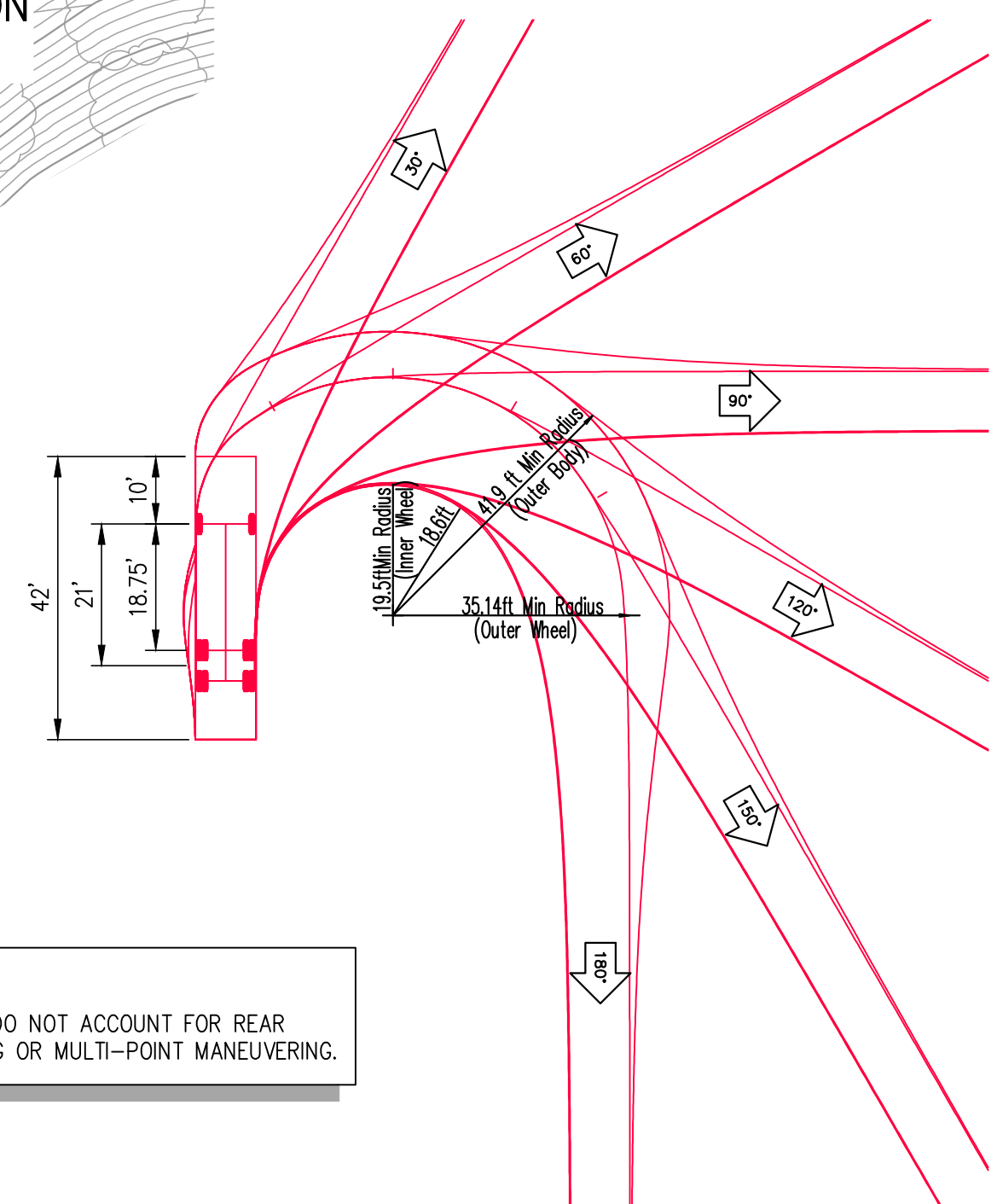
CITY OF NOVATO AERIAL LADDER FIRE TRUCK (NOT TO SCALE)
