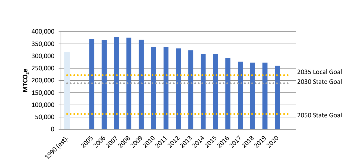
FIGURE 1: NOVATO GHG EMISSIONS AND TARGETS
