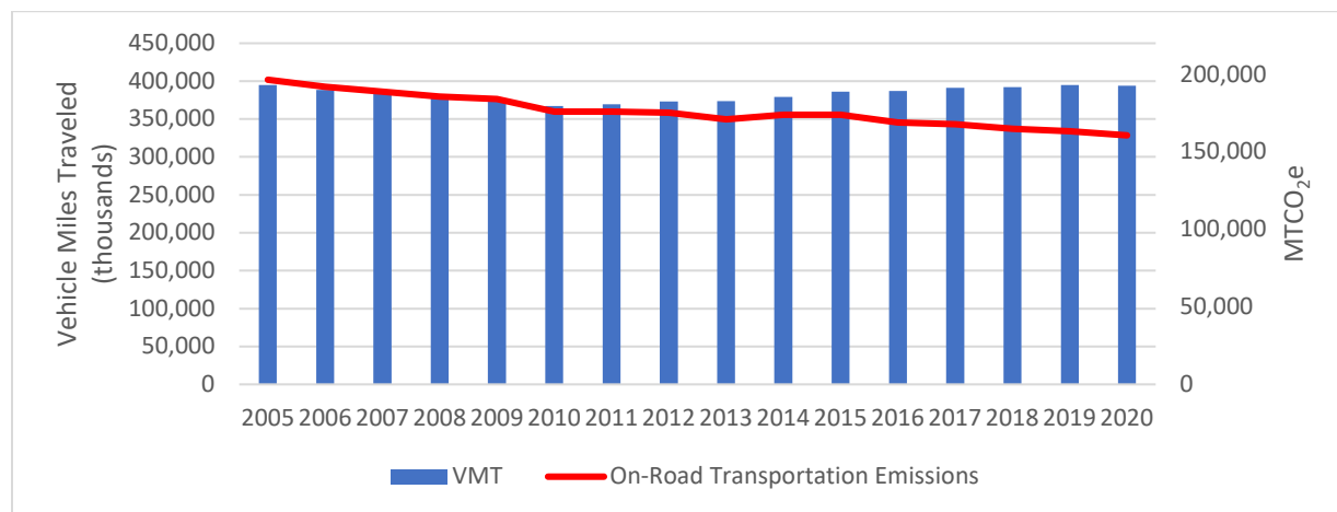
FIGURE 6: ON-ROAD VEHICLE MILES TRAVELED AND TRANSPORTATION EMISSIONS
