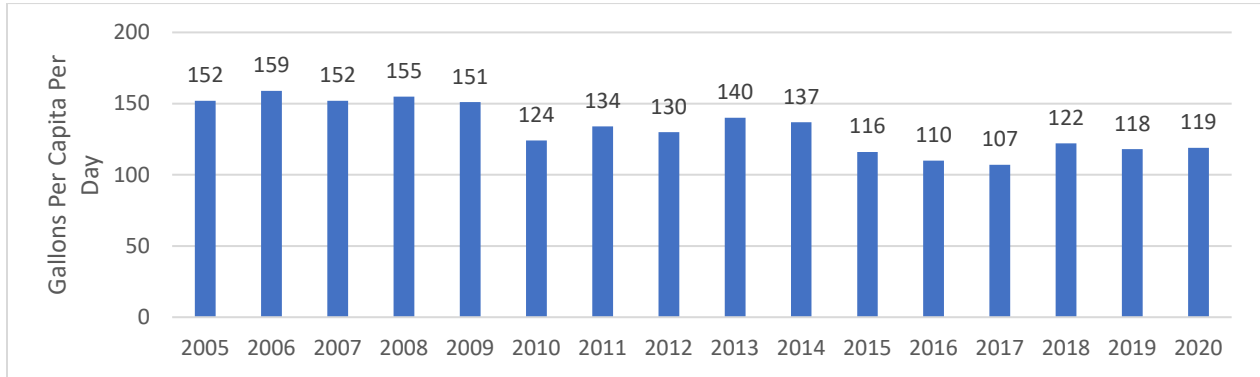
FIGURE 10: WATER USE AND EMISSIONS
