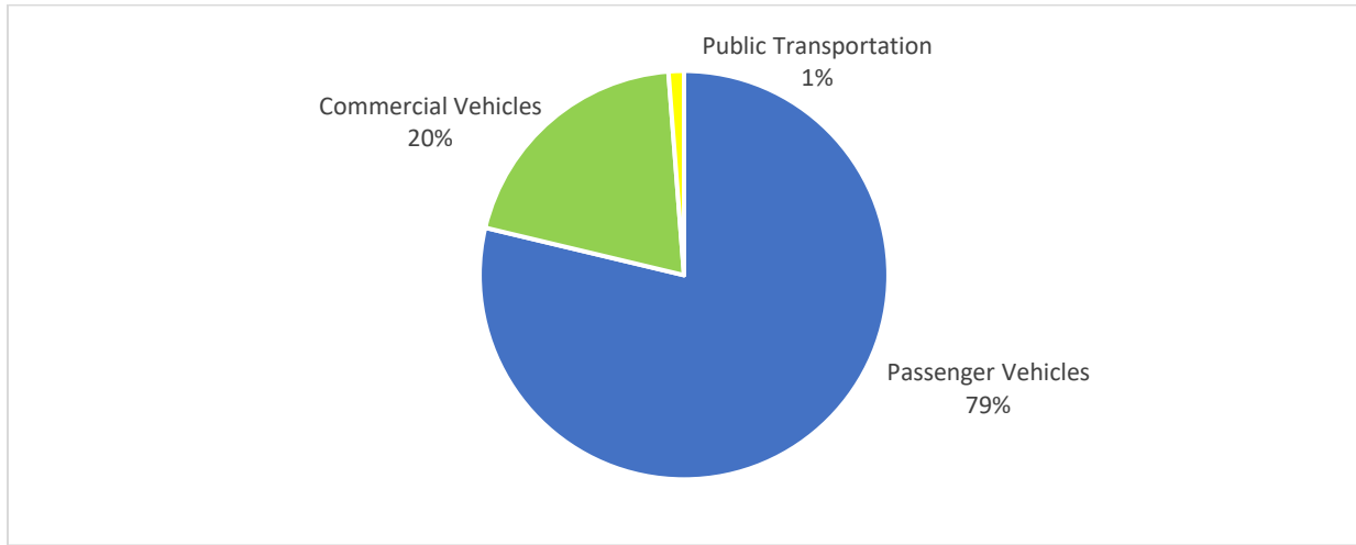
FIGURE 7: TRANSPORTATION EMISSIONS BY VEHICLE CATEGORY
