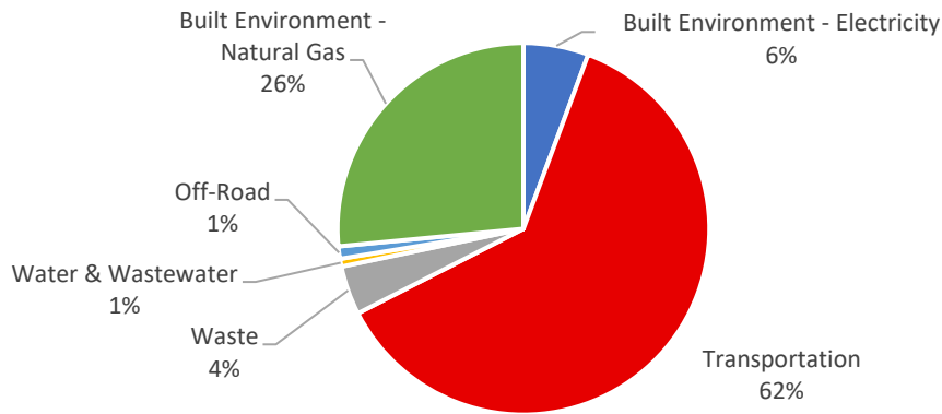
FIGURE 2: EMISSIONS BY SECTOR, 2020
